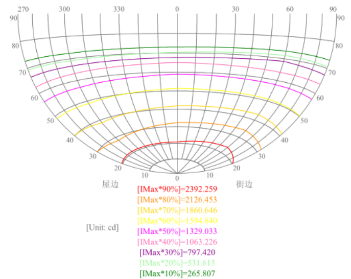
Round ISO Light Intensity Curve
